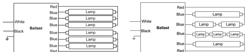
(3) 6-lamp wiring
